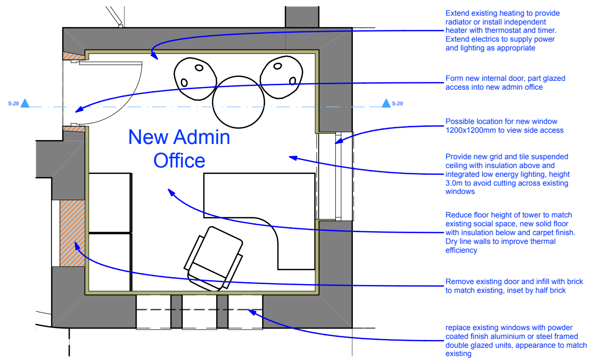
W-01 New admin office plan 1:50
